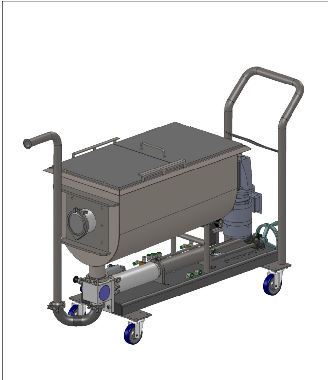
TEMPF-30-HOP MOBILE HOPPER CART (RENDER)
